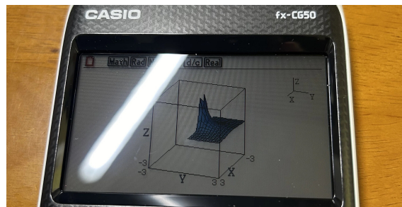
Completion of normed spaces, the graph of E = E(Y, X) , convolutions, and key inequalities.
